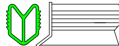
JOINT INTERSECTION PRIOR TO ASSEMBLY
