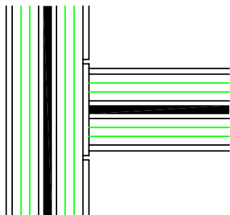
JOINT 3-WAY INTERSECTION PLAN
