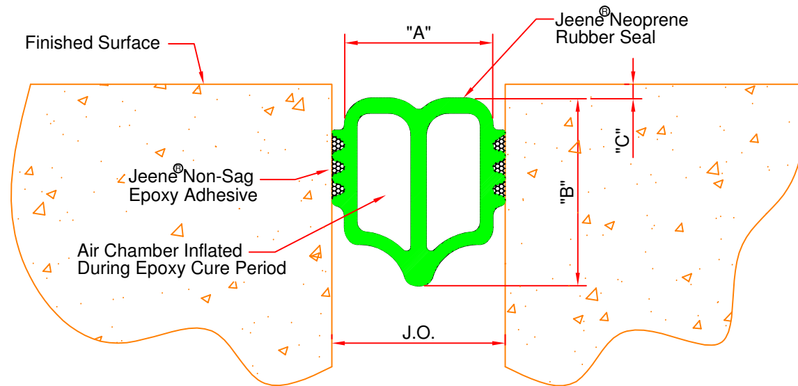
"FW" PROFILE SLAB-TO-SLAB CONDITION
